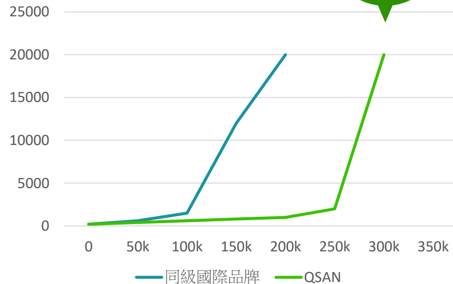
Random Write 4K Latency
